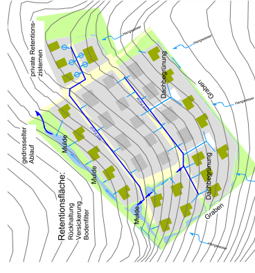
System Regenwassermanagement
